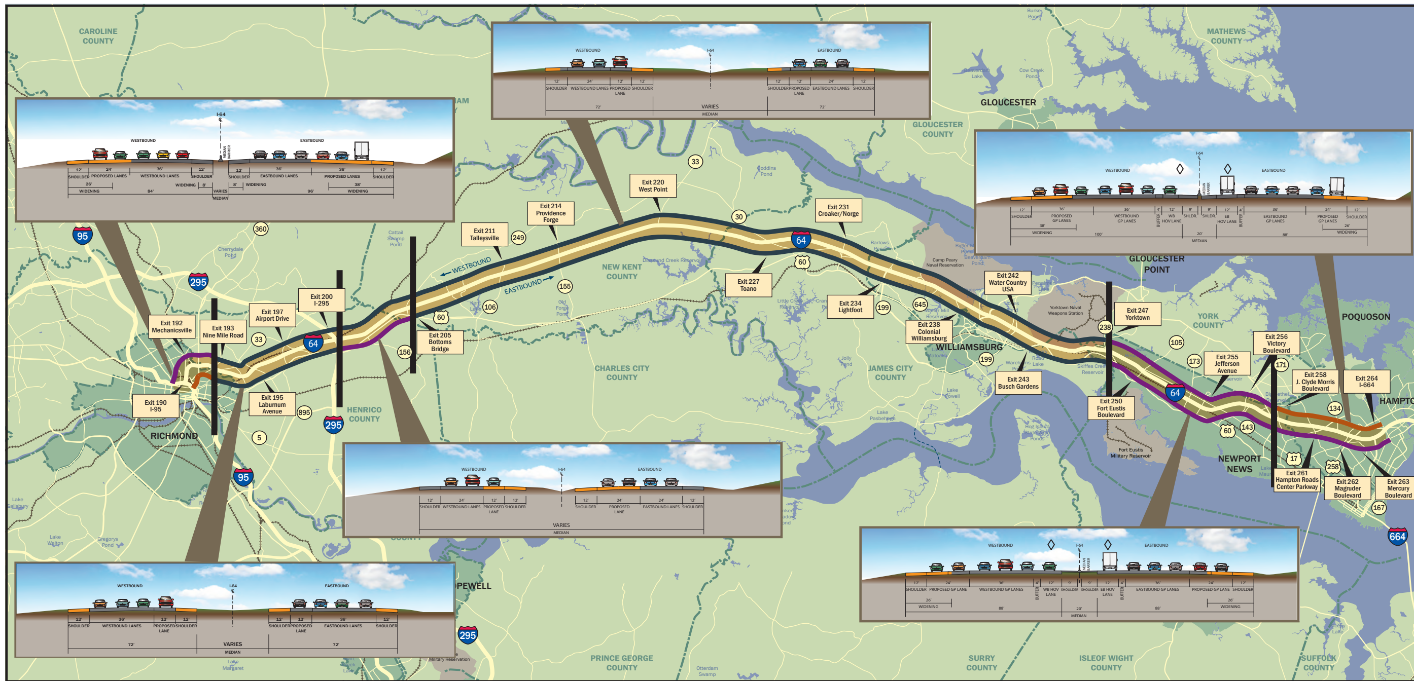
Figure II.4 Proposed Number of Additional Lanes for Build Alternatives 1B and 2B
