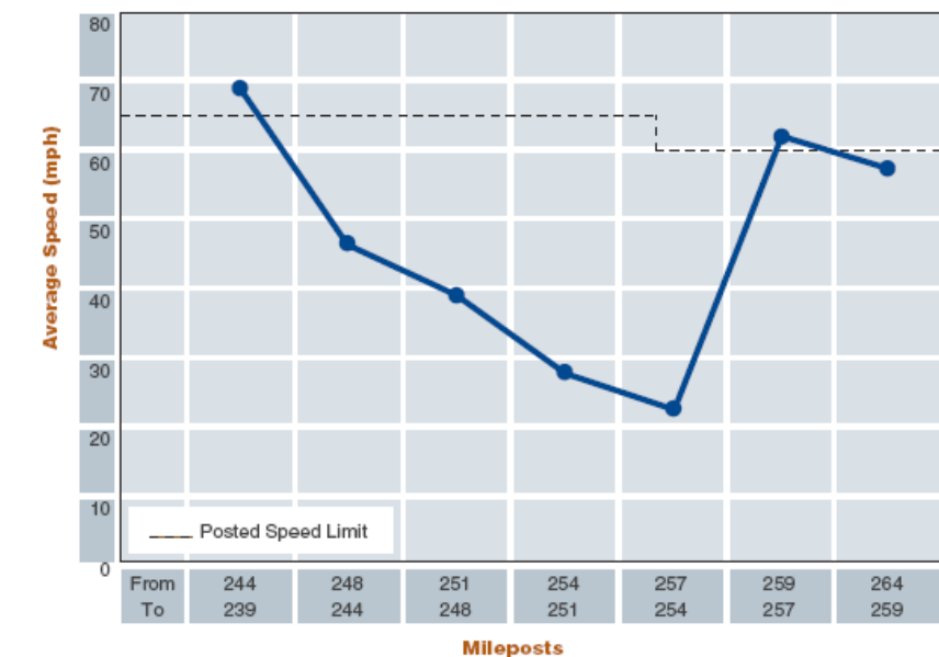
Figure I.3B: 2011 Average Travel Speeds Between Exit 239 and 264 (Westbound)
