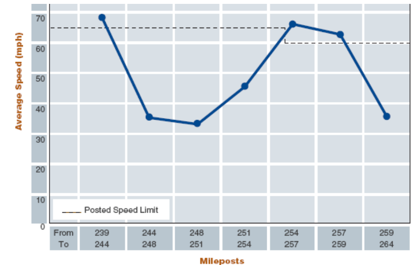
Figure I.3A: 2011 Average Travel Speeds Between Exits 239 and 264 (Eastbound)
