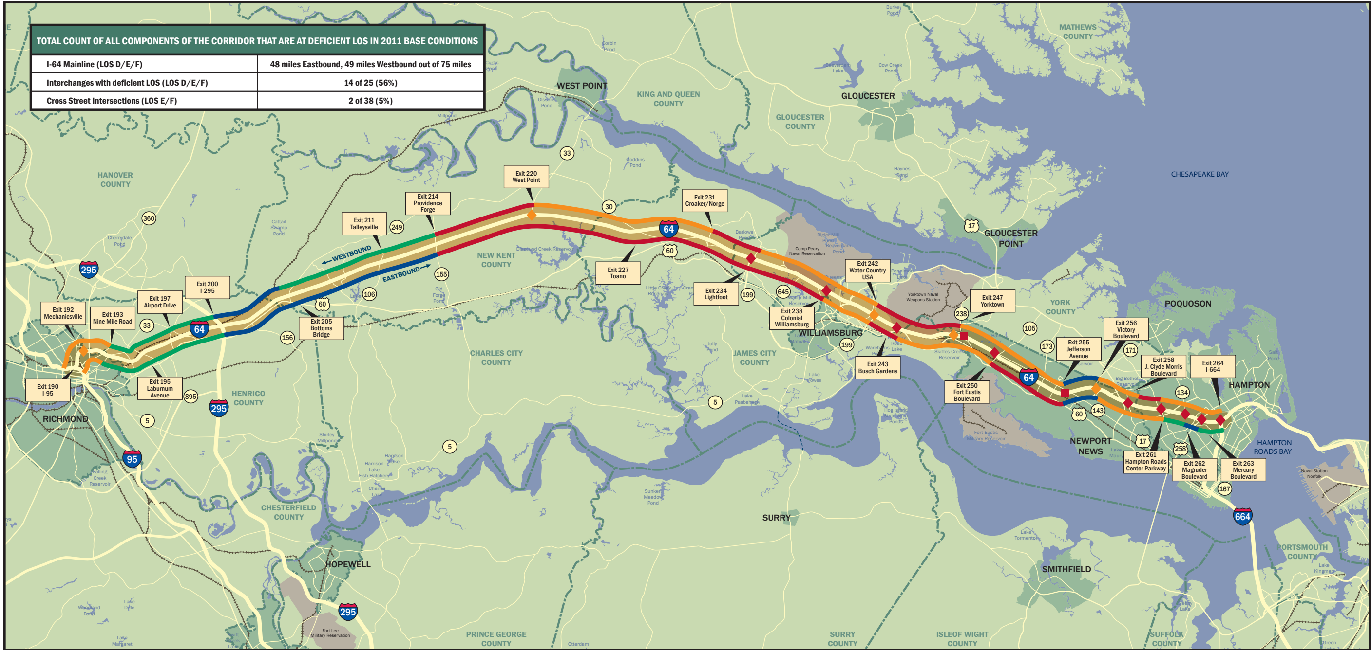
Figure I.4 I-64 Eastbound and Westbound Level of Service – Mainline and Deficient Ramp/Weave/Intersection 2011 Base Conditions
