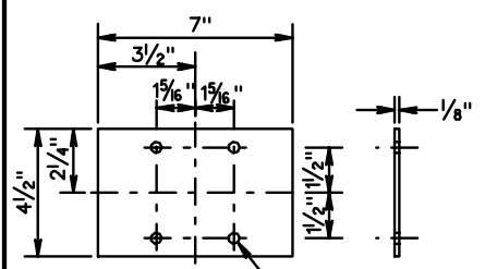
ANTI-TWIST PLATE
