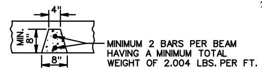
SECTION B-B TYPICAL BEAM SECTION
