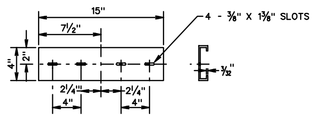
ADAPTER SHELF
